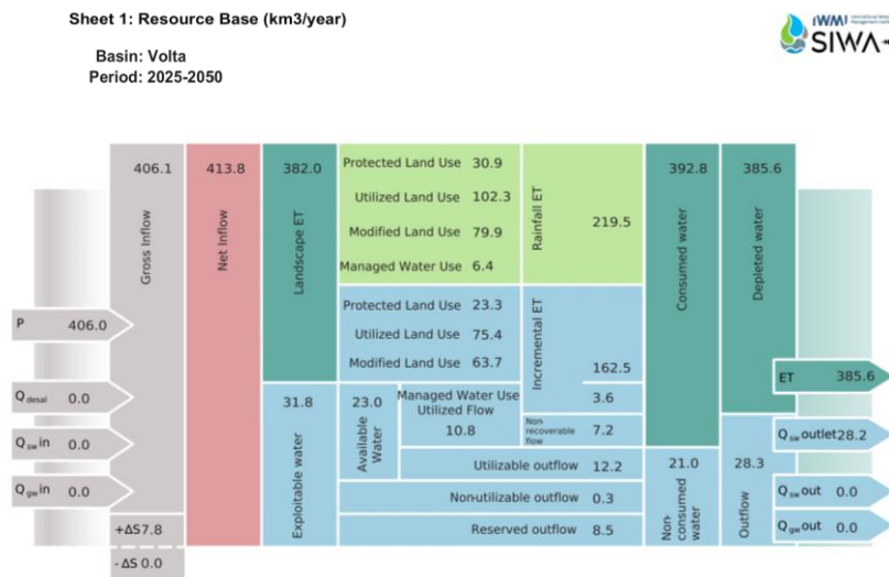
Figure 6: Water accounts for the Volta basin for the period 2025-2050 for the ensemble mean of GFDL-ESM4 Model and MPI-ESM1-2-HR Model.
