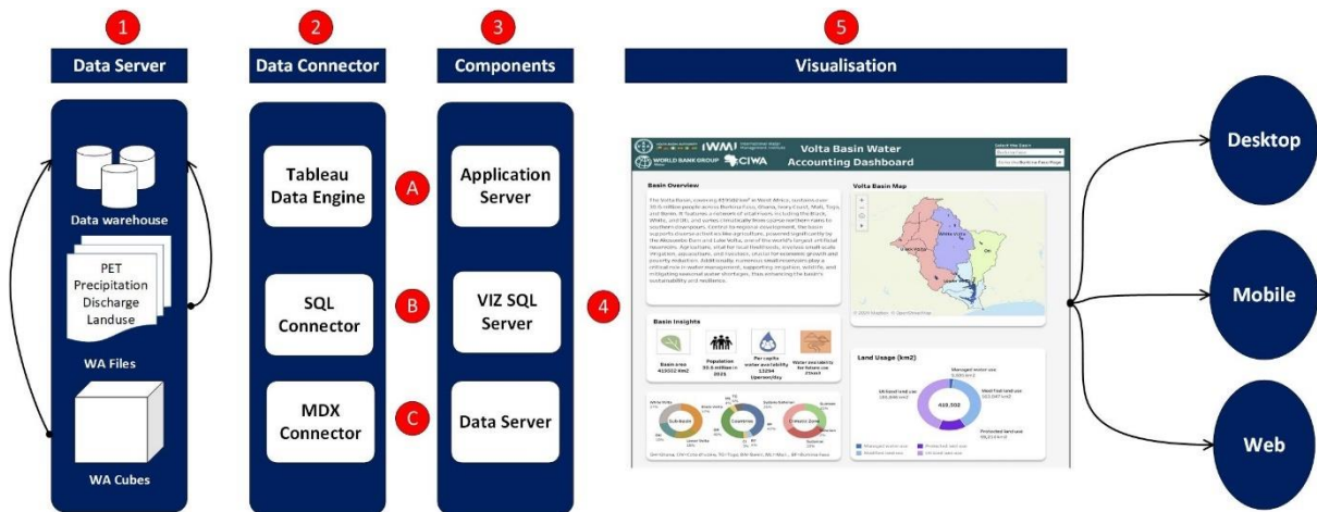
Figure 13. Tableau Architecture implemented.
